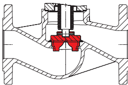
V-port regulating plug with marginal seat
