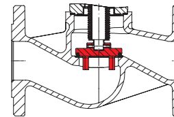
V-port plug with soft seal Max. operating temperature 392°F / 200°C at PTFE + 25% Kohle
