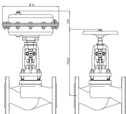
Pneumatic actuator ARI-FA Spring closes
