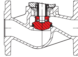
Regulating plug with soft seal Max. operating temperature 392°F / 200°C at PTFE + 25% Kohle
