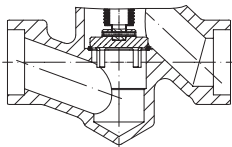
Fig. 149....153....3 / ....154....3 with socket weld ends
