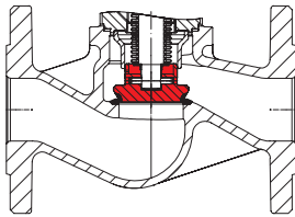
Isolation plug with marginal seat; stellite
