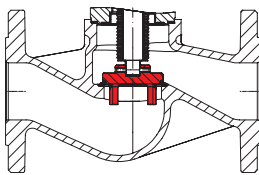
V-port plug with marginal seat; stellite
