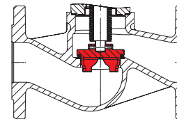
V-port regulating plug with soft seal Max. operating temperature 392°F / 200°C at PTFE + 25% Kohle
