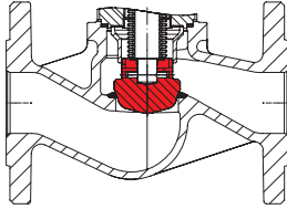
Isolation plug with marginal seat; stellite
